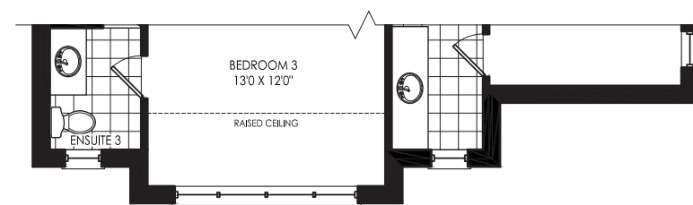
PARTIAL SECOND FLOOR ELEV 'B'
