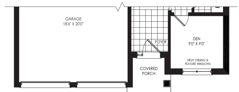
PARTIAL GROUND FLOOR ELEV 'B'
